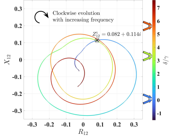
Fig. 1. Clockwise path traced by normalized Z_{12} in the complex impedance plane over a small frequency band. The color scale corresponds to the frequency difference \delta = f_a - f_b , where f_b is the first frequency at which Z_{12} is within the gray circle of radius \epsilon = 0.015 centered on Z_{12}^t = 0.082 + 0.114i . Here, \delta is normalized by a characteristic scale corresponding to the typical Q -widths of the modes \gamma = 2\alpha\Delta = 0.66 MHz, where \alpha is the RCM loss parameter and \Delta is the mean mode spacing. The arrows on the color bar mark the frequencies at which Z_{12} enters and leaves the circle. The impedance Z_{12} plotted in this figure is experimentally measured from a three-dimensional cavity with absorption \alpha = 5.5 .
