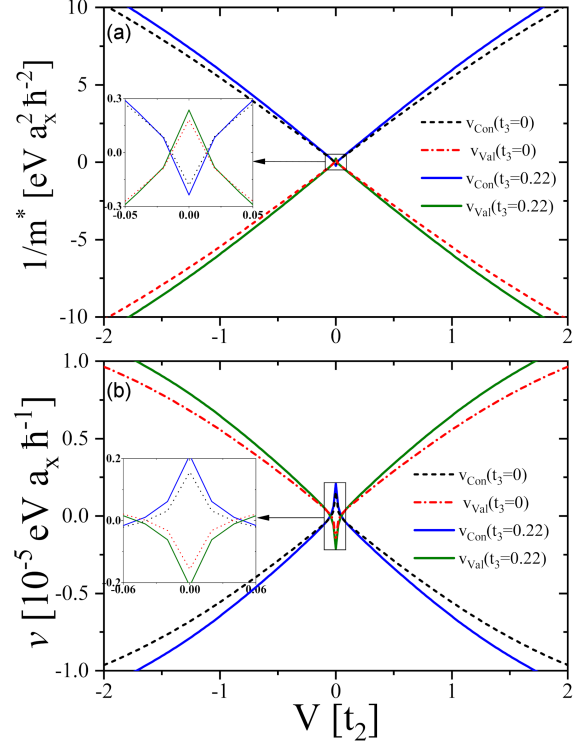
Fig. 8. Reciprocal effective mass (a) and velocity of carriers (b) in the highest valence band and lowest conduction band near the Fermi energy of ZBLPNRs with widths M = 16 as a function of the bias voltage.
