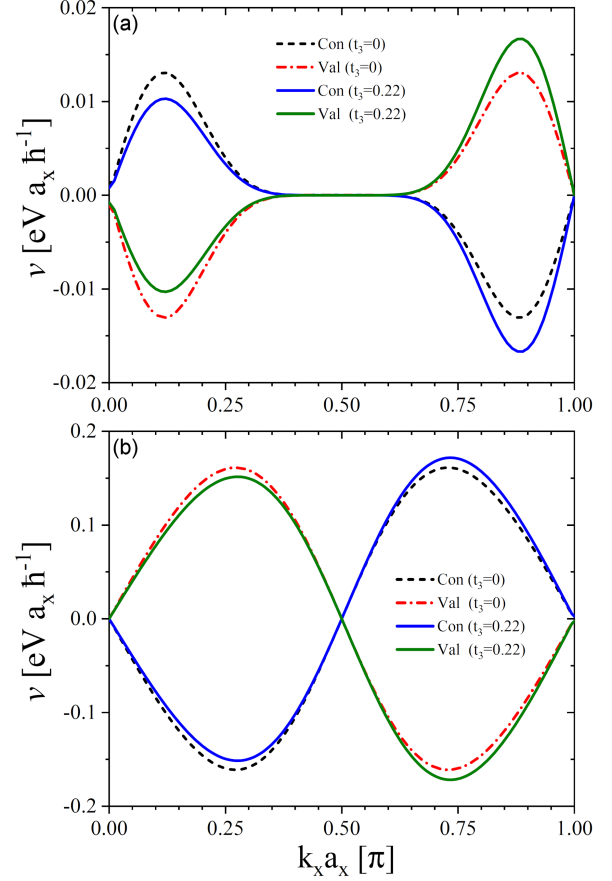
Fig. 6. The electron velocity in the highest valence band and the lowest conduction band near the Fermi energy for ZBLPNRs with M = 16 in the first Brillouin zone, with and without the interlayer hopping parameter t_3 . Panel (a) shows the result for zero electric field ( V = 0 ), and panel (b) for nonzero electric field ( V = 0.5 eV).
