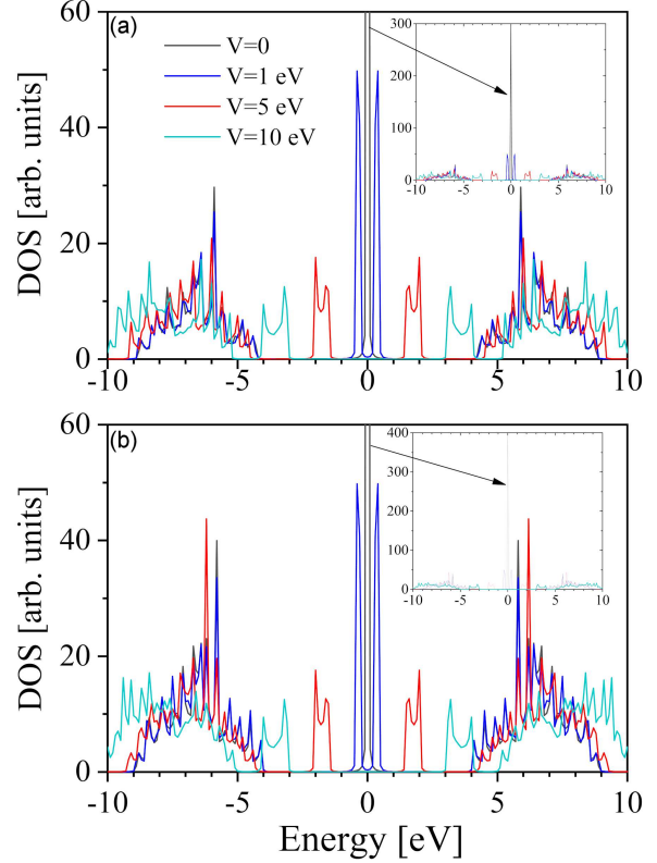
Fig. 5. Densities of states (DOS) calculated for (a) ZBLPNR with M = 12 and (b) ZBLPNR with M = 16 . For better clarity, DOSs around zero energy ( E = 0 ) are shown in the insets.
