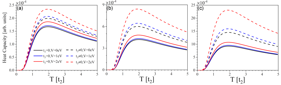
Fig. 9. Heat capacity of a ZBLPNR with M = 12 (a), M = 24 (b), and M = 48 (c) in terms of temperature for several values of electric potential V = 0, 1, 2 eV, in the absence ( t_3 = 0 ) and presence ( t_3 = 0.22 eV) of interlayer hopping parameter.
