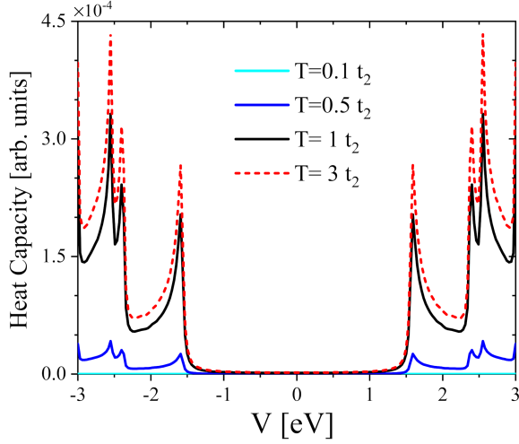
Fig. 10. Heat capacity of a ZBLPNR with M = 12 for four finite temperatures T/t_2 = 0.1, 0.5, 1, 3 , as a function of the electric potential.
