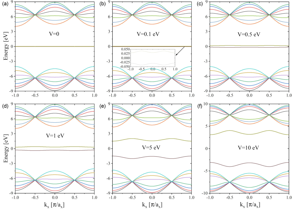
Fig. 2. The one-dimensional (1D) band structures of the system in Fig. 1 with (a-f) different external electric potential V , in which k_x is the wave vector parallel to the zigzag direction.
