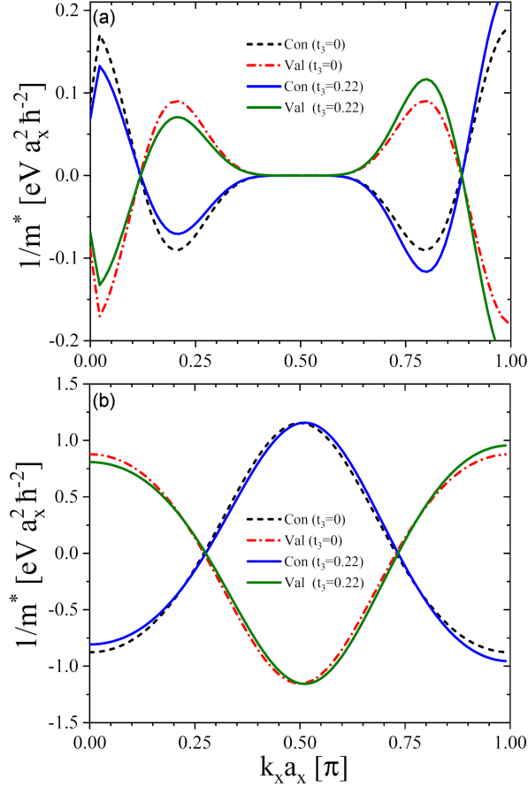
Fig. 7. The carrier reciprocal effective mass in the highest valence band and lowest conduction band near the Fermi energy for ZBLPNRs with M = 16 in the first Brillouin zone, with and without the interlayer hopping parameter, t_3 . Panel (a) shows the result for zero electric field ( V = 0 ), and panel (b) for nonzero electric field ( V = 0.5 \text{ eV} ).
