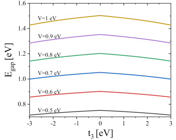
Fig. 4. Energy gap of bilayer phosphorene nanoribbons with widths M = 12 and 24 as a function of the interlayer hopping parameter t_3 for various bias voltage V .
