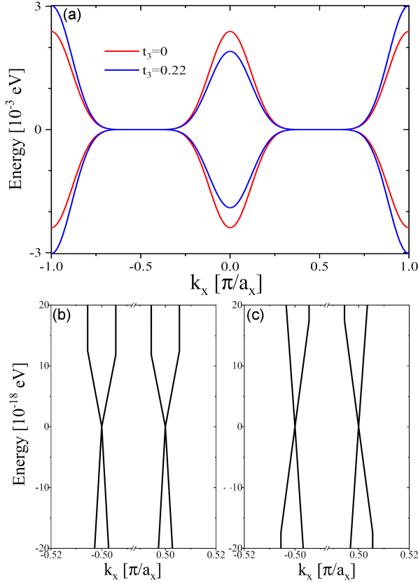
Fig. 3. (a) The highest valence band (HVB) and the lowest conduction band (LCB) for ZBLPNR with M = 16 , in the absence of the electric field ( V = 0 ) and with ( t_3 = 0 , red curve) and without ( t_3 = 0.22 eV, blue curve) the interlayer coupling. Panels (b) and (c) show a zoomed view of panel (a) for the highest and lowest bands near the zero Fermi energy in the vicinity of the high symmetry points k_x = \pm\pi/2 .
