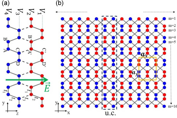
Fig. 1. Schematic illustration of zigzag bilayer black phosphorus nanoribbon with M = 16 — side view (panel a) and top view (panel b) — in the presence of a perpendicular electric field \mathbf{E} . The positions of the phosphorus atoms located in the bottom and top layers are presented by blue and red circles, respectively. The solid rectangle represents the unit cell of bulk bilayer phosphorene with the lattice constants a_x and a_y , and the dashed rectangle denotes the unit cell (u.c.) in the calculation of the tight-binding model of the nanoribbon.
