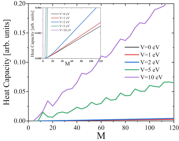
Fig. 11. The width dependence of the HC for ZBLPNRs for several values of electric potential V = 0, 1, 2, 5, 10 eV with T = t_2 .
