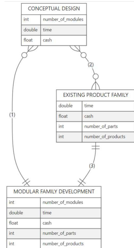
Fig. 7. Data exchange between conceptual and structural design and numerical comparison of design results with the pre-modularisation family.
