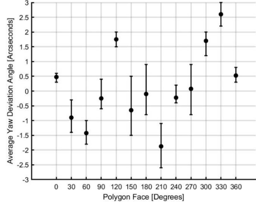
Fig. 2. Results obtained using two autocollimators and a 12-face polygon.
