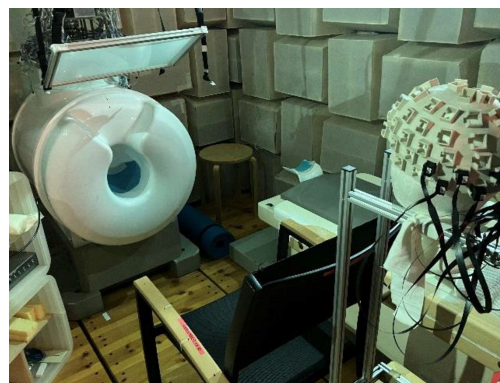
Fig. 1. Setup for magnetoencephalography with optically pumped magnetometers. OPMs are inserted in a MRI-derived 3D-printed sensor holder (right side of the photo). Participants are sitting in a chair and watching images on the tilted screen (left side of the photo).
