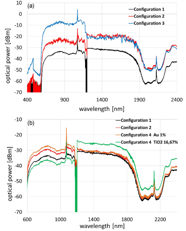
Fig. 7. Spectral characteristics in the transmission set-up — (a) configurations: 1 (black), 2 (red), 3 (blue); (b) configurations: 1 (black), 2 (red), 4 (1% Au yellow), 4 (16.67% \text{TiO}_2 green).
