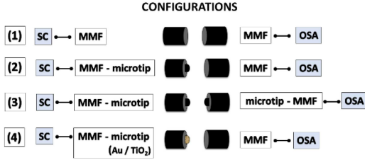
Fig. 6. Configurations of the microtip transmission properties testing system: (1) two MMF optical fibers, (2) a microtip on the transmitting fiber, (3) a microtip on the transmitting and receiving fibers, (4) a microtip doped with Au and \text{TiO}_2 on the transmitting fiber; SC — light source; OSA — spectrum analyzer.
