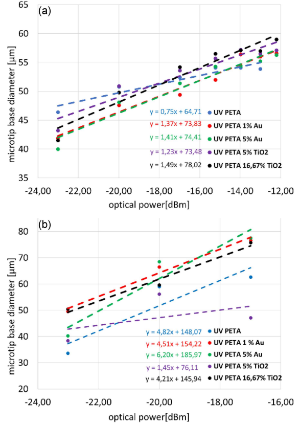
Fig. 2. Microtip base diameter vs optical power for UV PETA mixture and: (a) MMF 62.5 \mu\text{m} , (b) MMF 105 \mu\text{m} .
