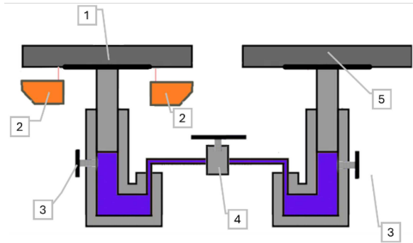
Fig. 2. Schematic diagram of the test stand; 1 — pressure balance standard, 2 — laser sensors, 3 — shut-off valves, 4 — pressure pump, 5 — pressure balance under test.
