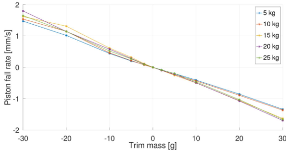
Fig. 7. Fall rate of the piston [mm/s] vs trim mass [g] with separated total mass series.
