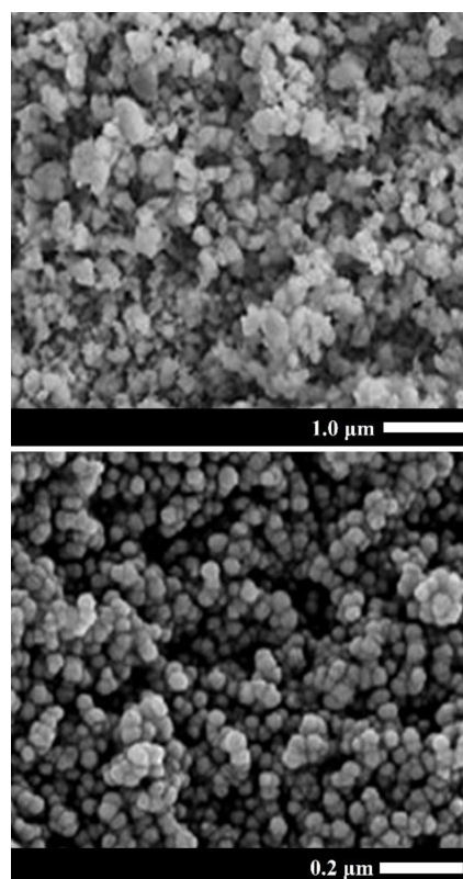
Fig. 2. SEM images of synthesized AgNPs.
