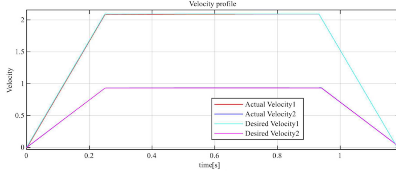
Fig. 12. Velocity tracking accuracy using OSOSMC.
