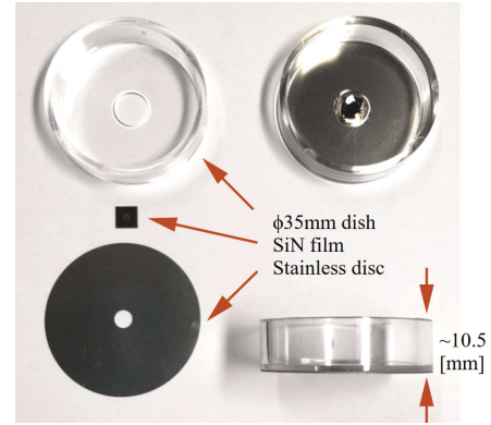
Fig. 3. Standard 35 mm D-EXA ASEM dish.
