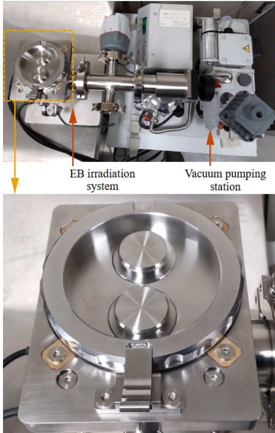
Fig. 11. Experimental 2-position fast sample switching turret assembly. Shown with two Ø35 mm covers installed.
