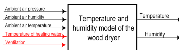
Fig. 1. Block diagram of the temperature and humidity model of the wood dryer.
