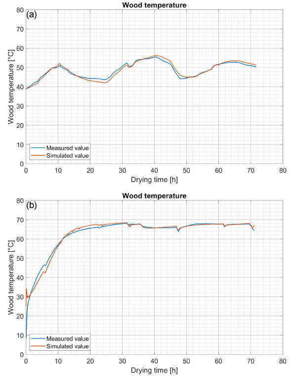
Fig. 5. Measured and simulation-derived change in wood temperature during drying of batches 1 and 2. The waveforms for batch 1 are shown in (a), and for batch 2 in (b).
