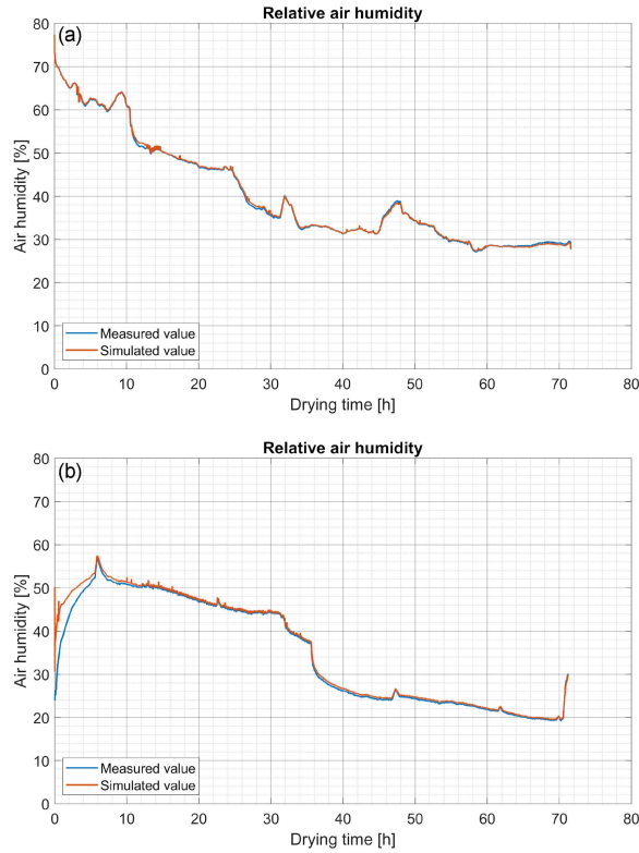
Fig. 3. Measured and simulation-derived change in relative humidity in the drying chamber during drying of batches 1 and 2. The waveforms for batch 1 are shown in panel (a), and for batch 2 in (b).
