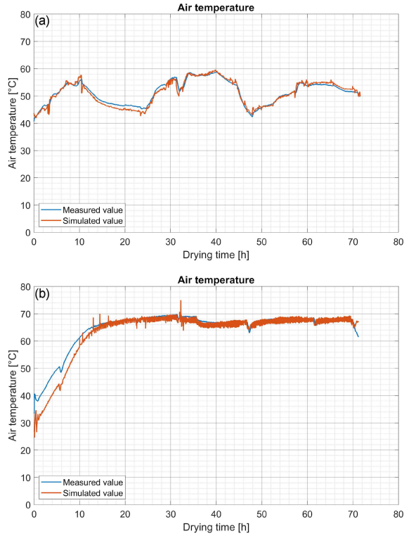
Fig. 4. Measured and simulation-derived temperature change in the drying chamber during drying of batches 1 and 2. The waveforms for batch 1 are shown in (a), and for batch 2 in (b).
