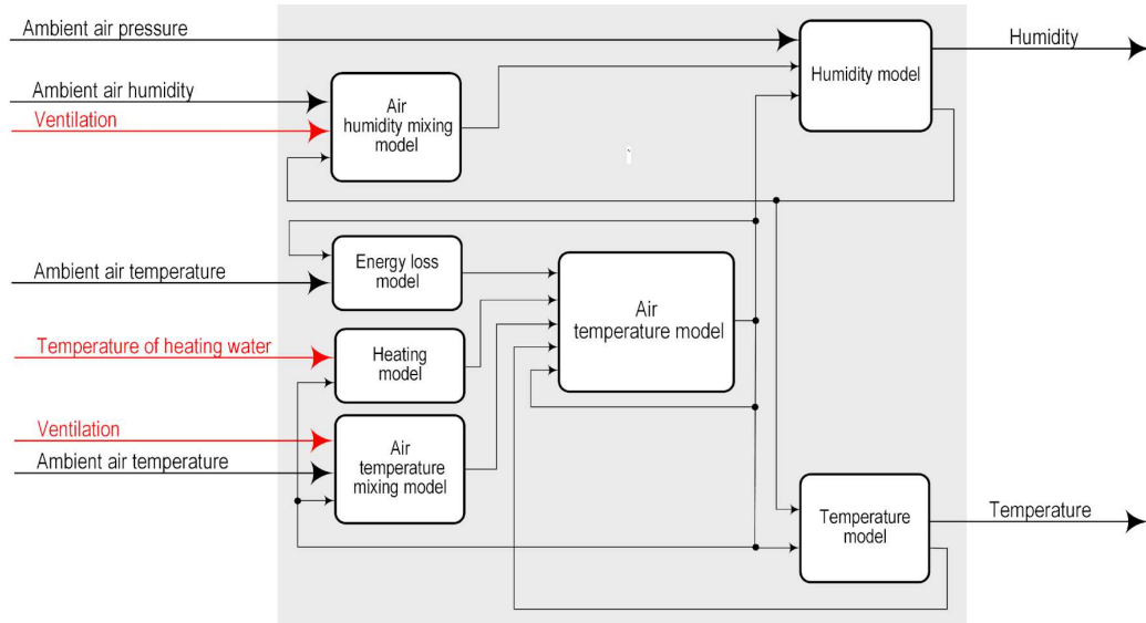
Fig. 2. Structure of the temperature and humidity model of the wood dryer.
