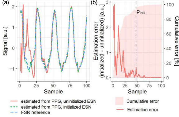
Fig. 3. Illustration of p_{\text{init}} : (a) FSR signal estimation from uninitialized vs initialized ESN and (b) corresponding absolute estimation error and the p_{\text{init}} index position ( N_{\text{init}} = 100 , \beta = 0.95 ).
