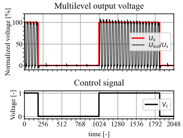
Fig. 1. Output voltage of a pulse generator.
