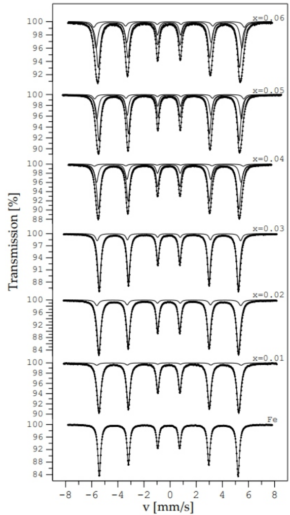
Fig. 2. The ^{57}\text{Fe} Mössbauer spectra for the \text{Fe}_{1-x}\text{Rh}_x alloys measured at room temperature after the annealing process at 1270 K and slow cooling to room temperature.
