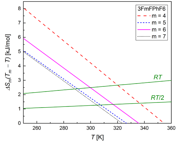
Fig. 7. Comparison of \Delta G = (T_m - T)\Delta S_m [25], with thermal energy of two translational degrees of freedom within the smectic layers. The T_m and \Delta S_m values were taken from [24].
