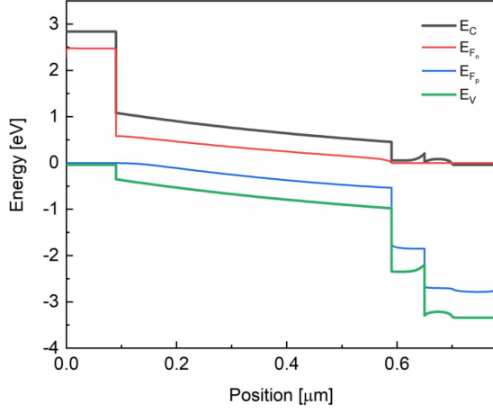
Fig. 3. Energy band diagrams of the proposed antimony selenosulfide-based device.
