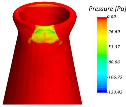
Fig. 7. The negative pressure over the spout produced by pouring liquid (flow rate of 0.2 l/min). Only negative pressures are considered. Positive pressure is shown in red.
