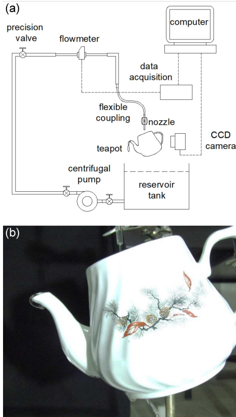
Fig. 1. (a) Experimental setup, (b) the teapot used in the experiments.
