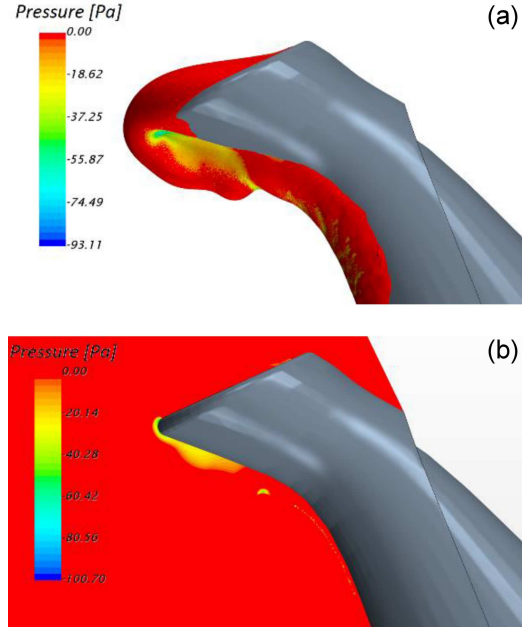
Fig. 6. The negative pressure of pouring liquid from the teapot (flow rate of 0.2 l/min) at (a) the free surface of the liquid as an iso-surface and (b) mid-plane. Only negative pressures are considered. Positive pressure is shown in red.
