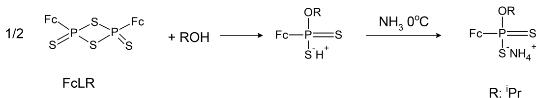
Fig. 2. Synthesis of the ammonium ferrocenyl dithiophosphate (1).
