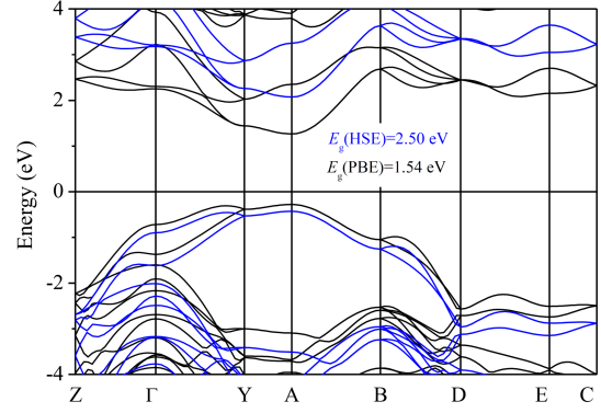
Fig. 4. Band structure of C2/c -C32 at the PBE (black lines) and HSE06 (blue lines) level.
